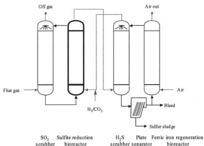
Figure 1. Combined chemical/biological process for conversion of \text{SO}_2 to \text{H}_2\text{S} .
