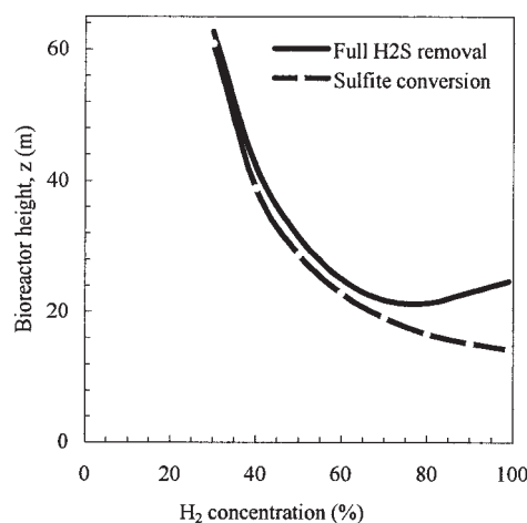
Figure 10. Effect of inlet gas \text{H}_2 concentration on the bioreactor height at constant total gas pressure; the height required for \text{H}_2\text{S} stripping equals the height for full \text{H}_2\text{S} removal minus the height required for sulfite conversion.
